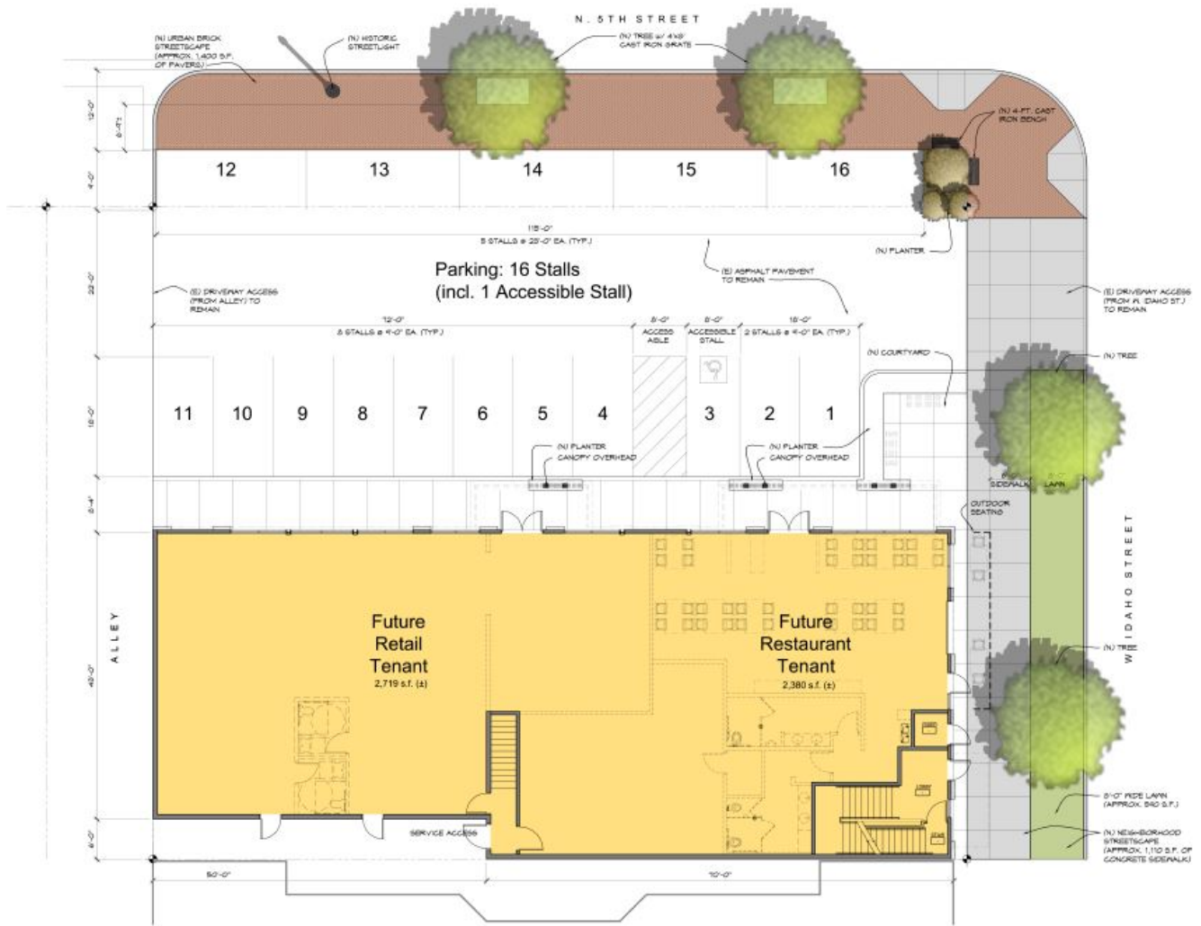
1 GROUND FLOOR / SITE - ALTERNATE OPTION 1/2" = 1'-0"
